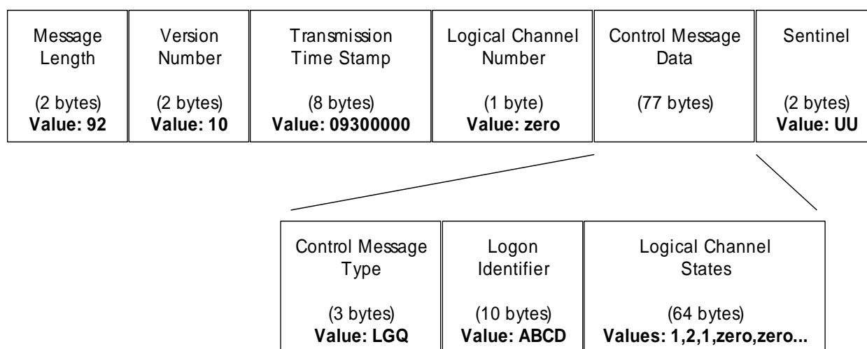
Figure Appendix A- 4 Logon control message, channel zero, 9:30 a.m.
